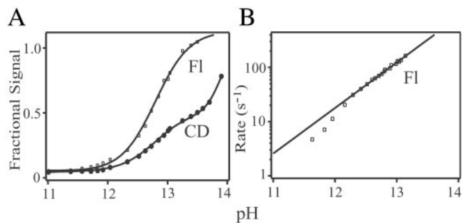
Fig. 3. High pH denaturation of Cyt c (no urea). (A) Above pH 12, denaturation occurs in two steps with a populated intermediate. A partial unfolding removes 45% of the CD 222 of the native protein and recovers all of the fluorescence of the U state (corrected for Trp pH titration and quenching). Both probes show the same midpoint (pK 12.8) and slope (1.5). Equilibrium unfolding to U occurs above pH 13. (B) The kinetics of intermediate formation. The black curve in Fig. 5A is constructed from FI data in 1.3 M urea. The zero urea data are shown here because CD 222 is obscured in high pH urea.
