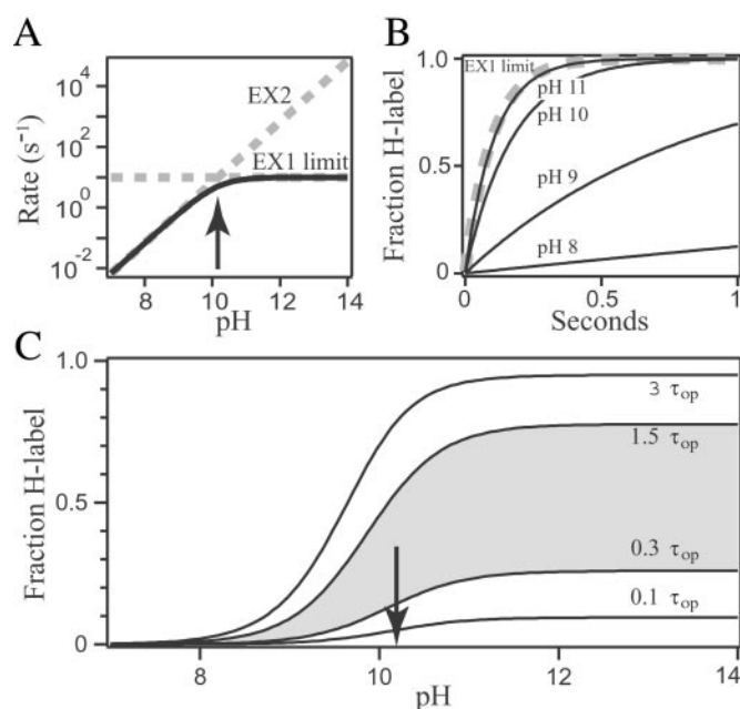
Fig. 2. Simulated HX results. (A and B) At low pH where exchange is in the EX2 limit, HX rate increases 10-fold for each pH unit. At high pH, HX rate limits at k_{\text{op}} (EX1 limit). (C) Simulation of expected curves when the HX exposure time is kept constant and pH is varied ( k_{\text{op}} = 10 \text{ s}^{-1} , k_{\text{cl}} = 10^4 \text{ s}^{-1} , k_{\text{int}} = 10^8 \text{ s}^{-1} ). The arrow shows the EX2 to EX1 transition point ( k_{\text{ch}} = k_{\text{cl}} ). An experimental curve in the gray region most sensitively measures the opening/closing parameters. At high pH, a different EX1 pattern can be produced when k_{\text{op}} increases with pH (black line in Fig. 5).
